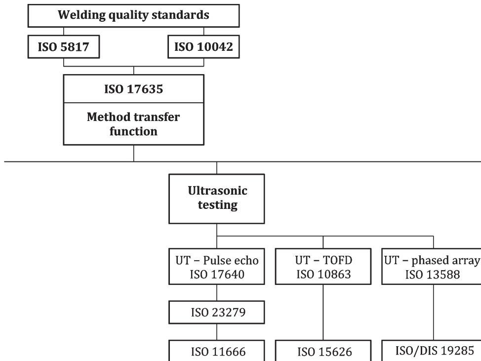
Figure B.3 — Graph of standard context for ultrasonic testing
