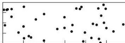
Figure A.4 — 2,5 surface percent, 38 pores, d = 1 mm
